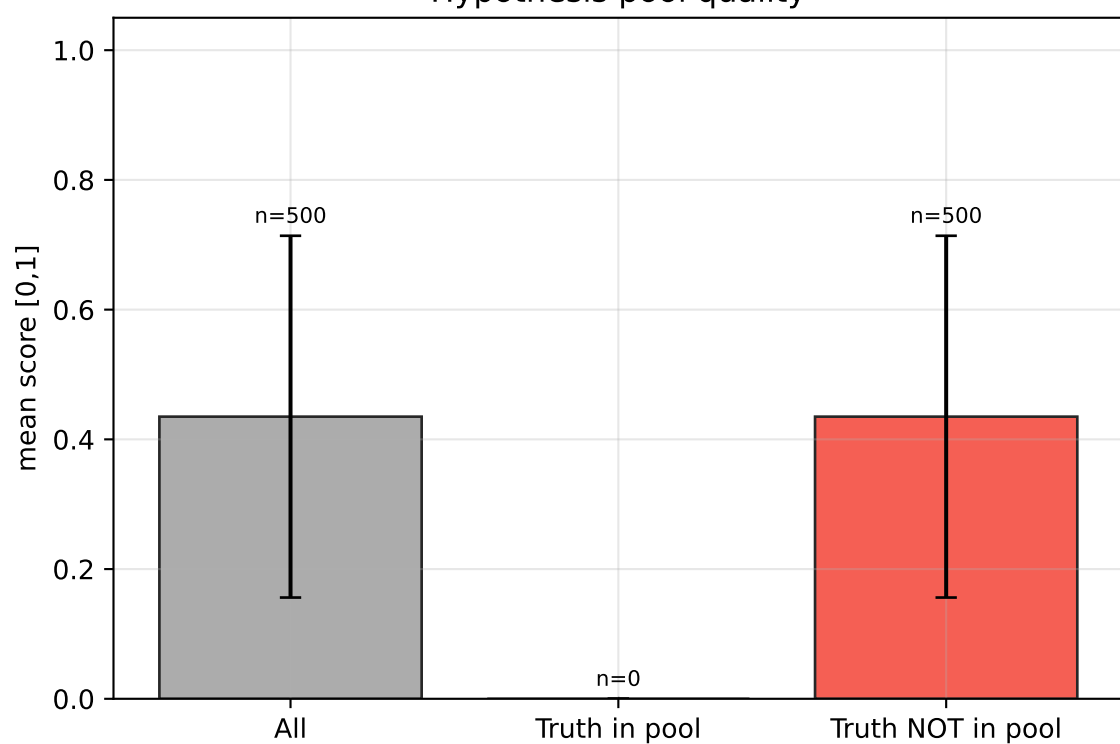
Hypothesis pool quality
